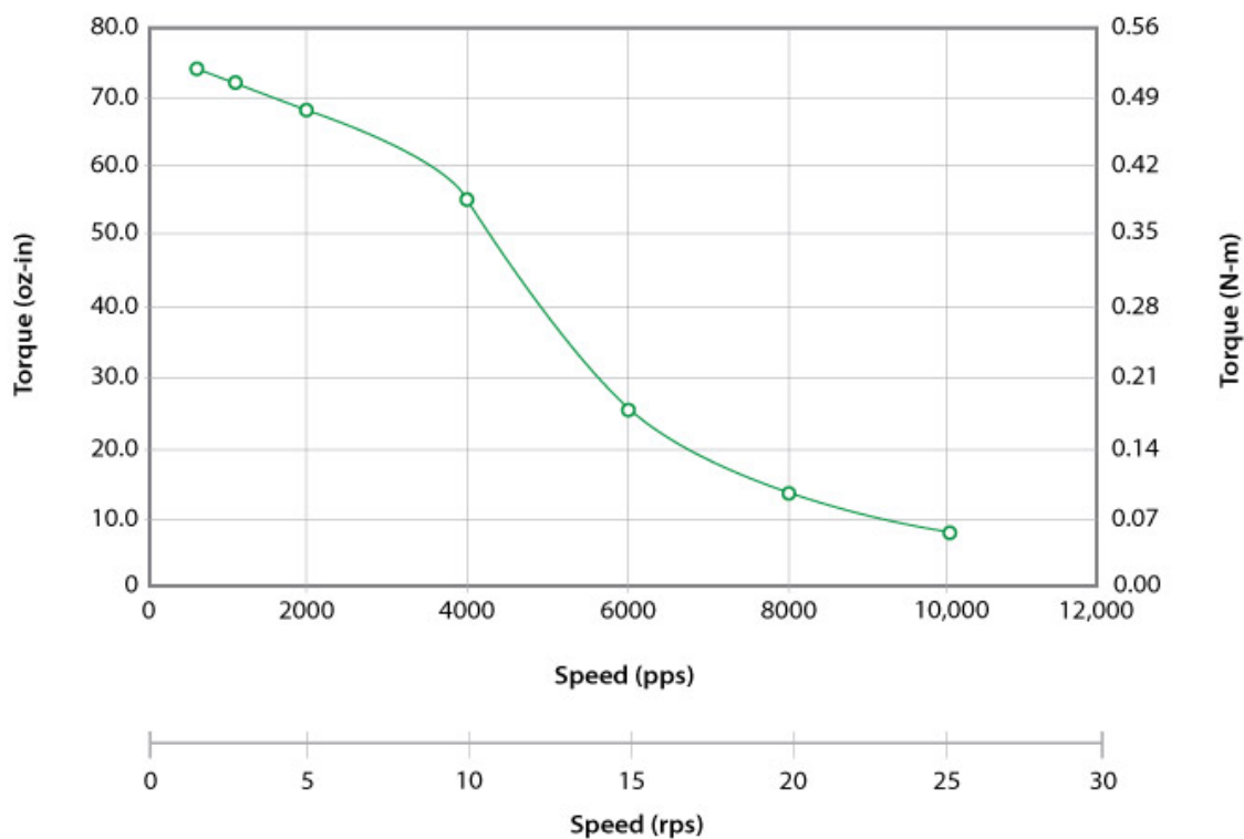
G4518L-01 24VDC, 2.0 Amps/Phase, Bipolar, 1/2 Stepping
